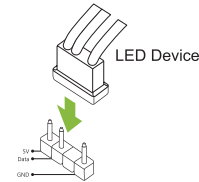
ARGB LED Device Header (5V_LED)
